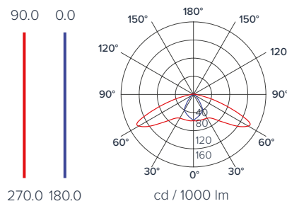
Photometric diagram GEMMA-C
